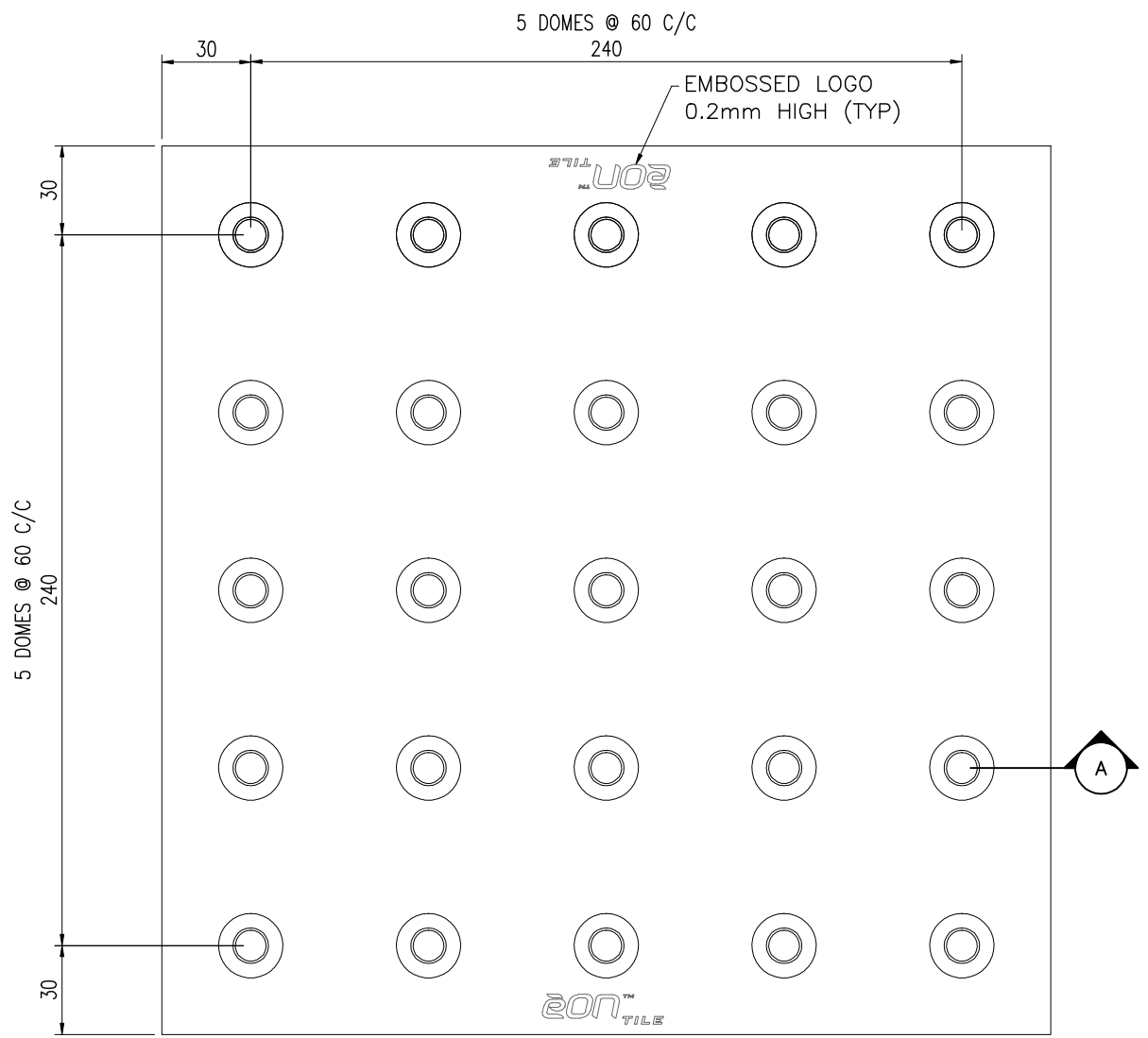
PLAN VIEW SCALE: 1:2.5
